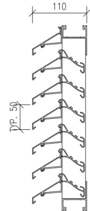
SECTION VIEW
